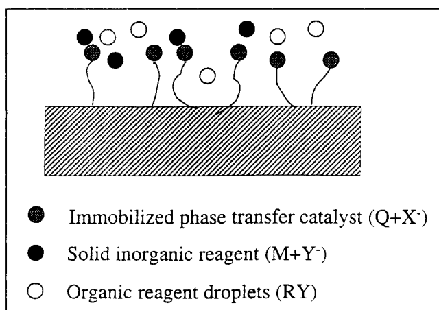
Figure 14. Plausible mechanism for liquid-solid-solid triphase catalysis.
