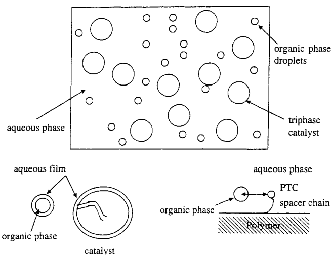
Figure 12. Plausible mechanism for liquid-liquid-solid triphase catalysis.
