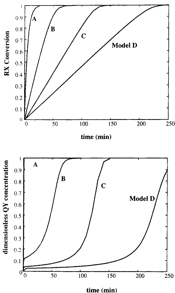
Figure 10. Comparison of models for homogeneous solubilization.
